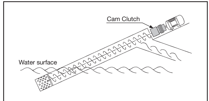
Figure 31: Inclined pump – Medium Overrunning Application
