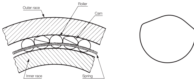
BS Series Cam Clutch construction and cam profile
