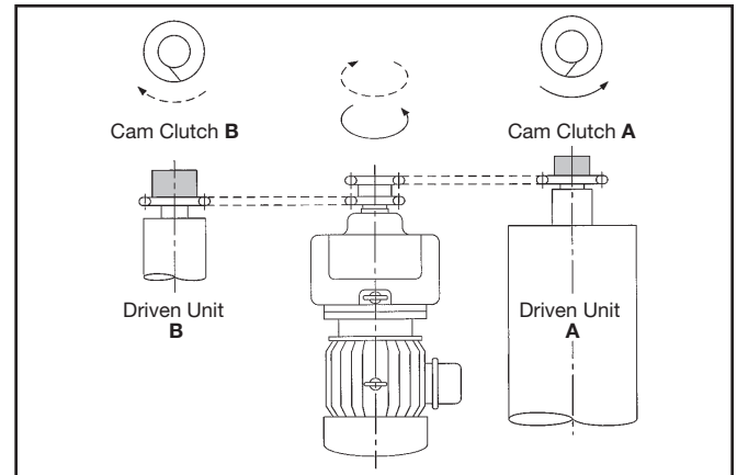
Figure 33: Selection based upon rotation direction
