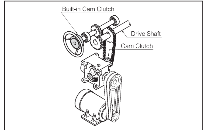
Figure 30: Common manual operation arrangement
