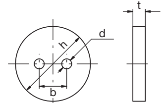
End Plate
