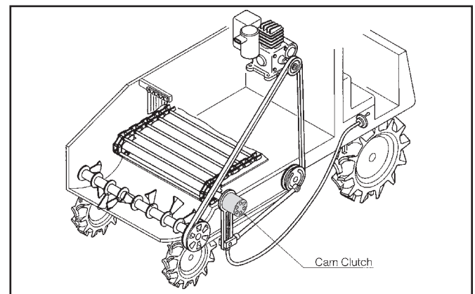
Figure 20: Manure Spreader
