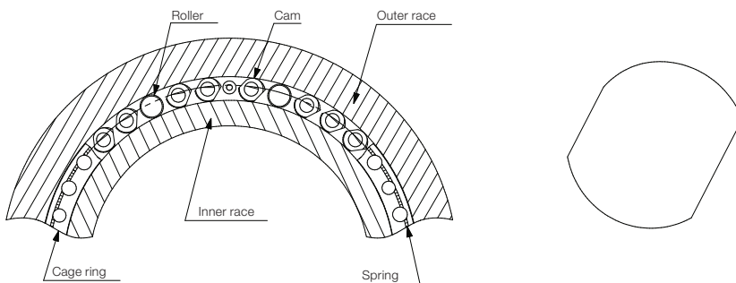
BS-F Series Cam Clutch construction and Non-rollover cam design
