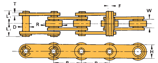
Double Pitch Type – Oversize roller type
