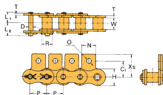
SA-1 Attachment
