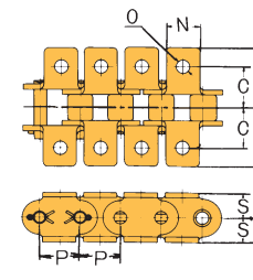
KK-1 Attachment
