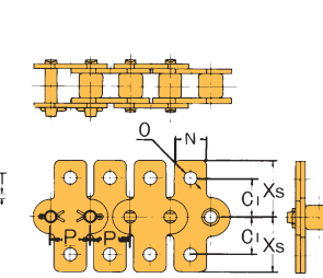
SKK-1 Attachment
